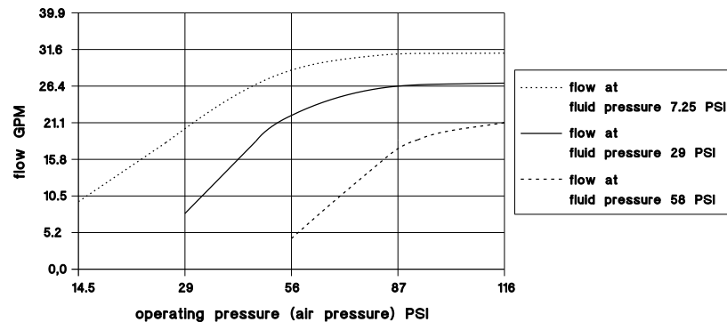
characteristic diagram UMP40: viscosity 138 SUS
