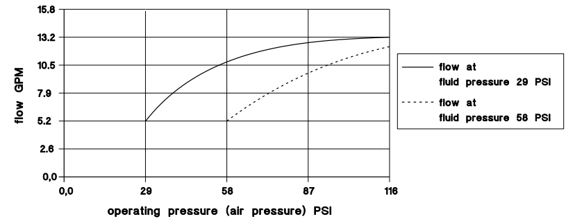
characteristic diagram UMP40: viscosity 460 SUS
